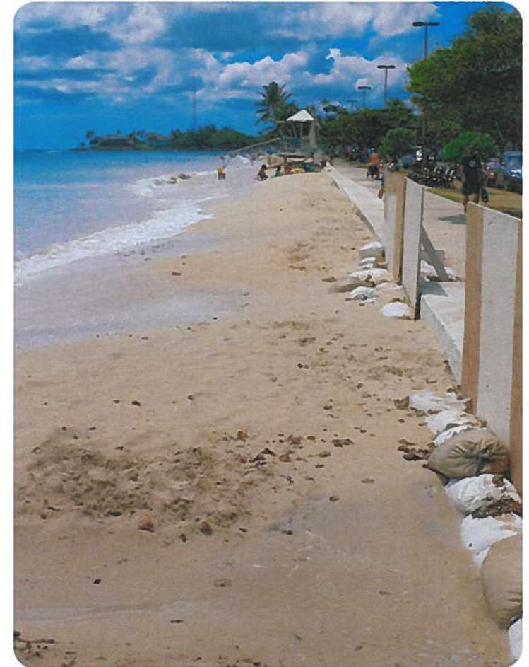
Temporary erosion protection at Ala Moana Beach Park.
