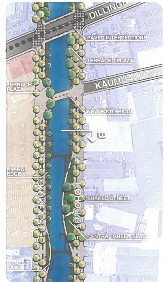
Canal improvements (Source: Kapālama Canal Master Plan)
